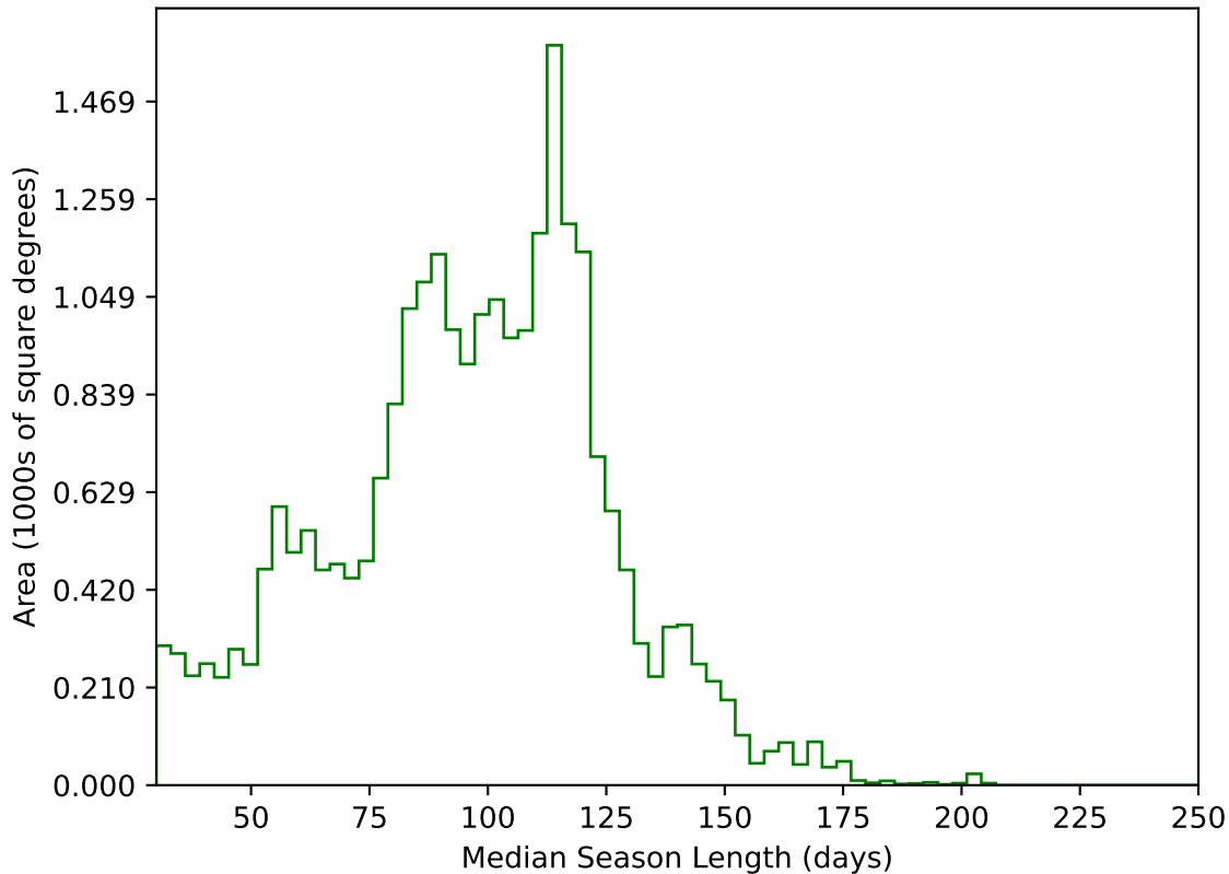
ddf_acor_sf20_lsf30_lsr50_v3.4_10yrs All sky g band: Median Season Length
