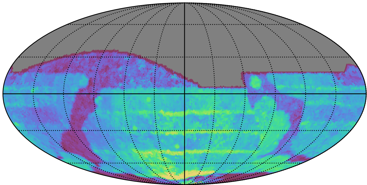
ddf_acor_sf20_lsf30_lsr50_v3.4_10yrs All sky all bands: Median Season Length
