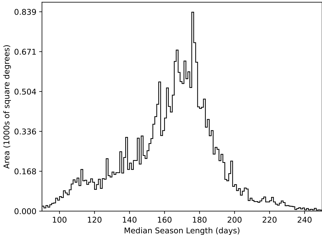
ddf_acor_sf20_lsf30_lsr50_v3.4_10yrs All sky all bands: Median Season Length
