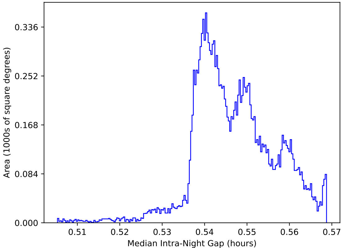
ddf_acor_sf20_ls30_lsr50_v3.4_10yrs WFD: Median Intra-Night Gap
