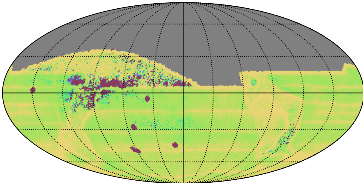
ddf_acor_sf20_lsf30_lsr50_v3.4_10yrs All sky: Median Intra-Night Gap
