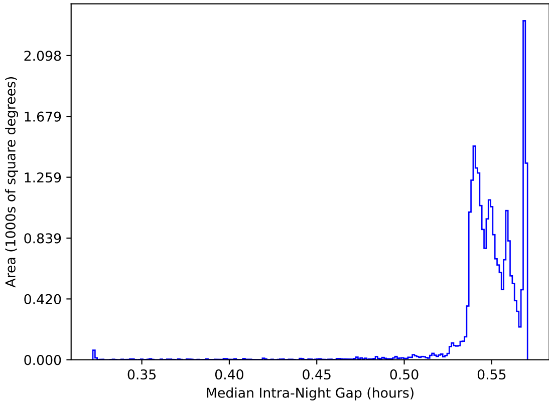
ddf_acor_sf20_lsf30_lsr50_v3.4_10yrs All sky: Median Intra-Night Gap
