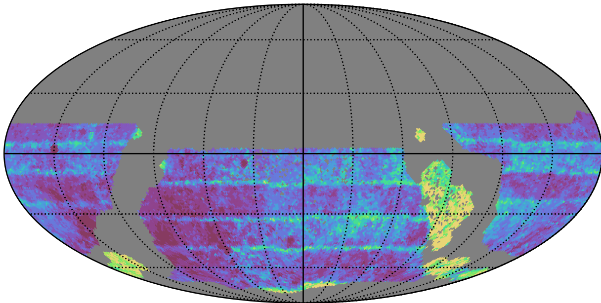
ddf_acor_sf20_lsf30_lsr50_v3.4_10yrs WFD z band: Median Inter-Night Gap
