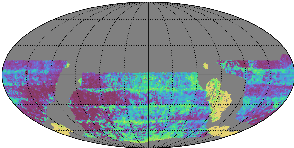
ddf_acor_sf20_lsf30_lsr50_v3.4_10yrs WFD y band: Median Inter-Night Gap
