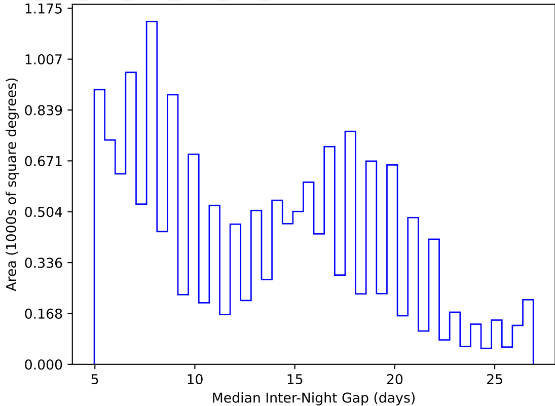
ddf_acor_sf20_lsf30_lsr50_v3.4_10yrs WFD y band: Median Inter-Night Gap
