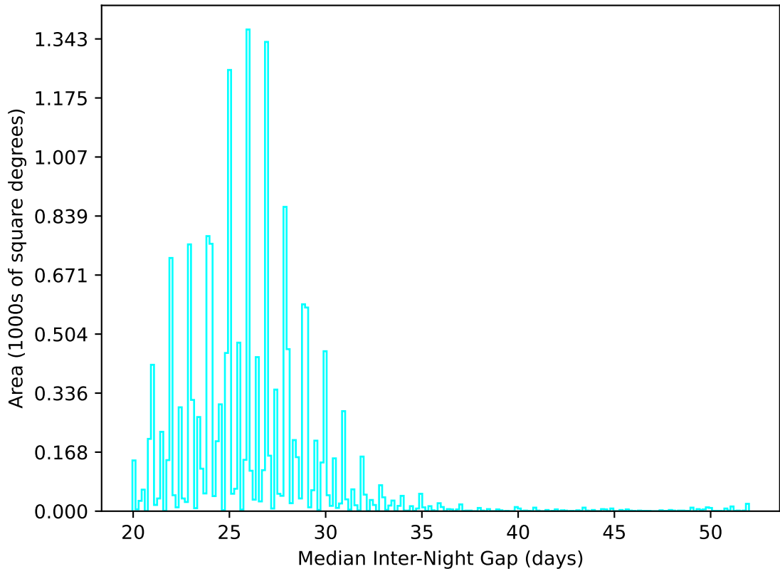
ddf_acor_sf20_lsf30_lsr50_v3.4_10yrs WFD u band: Median Inter-Night Gap
