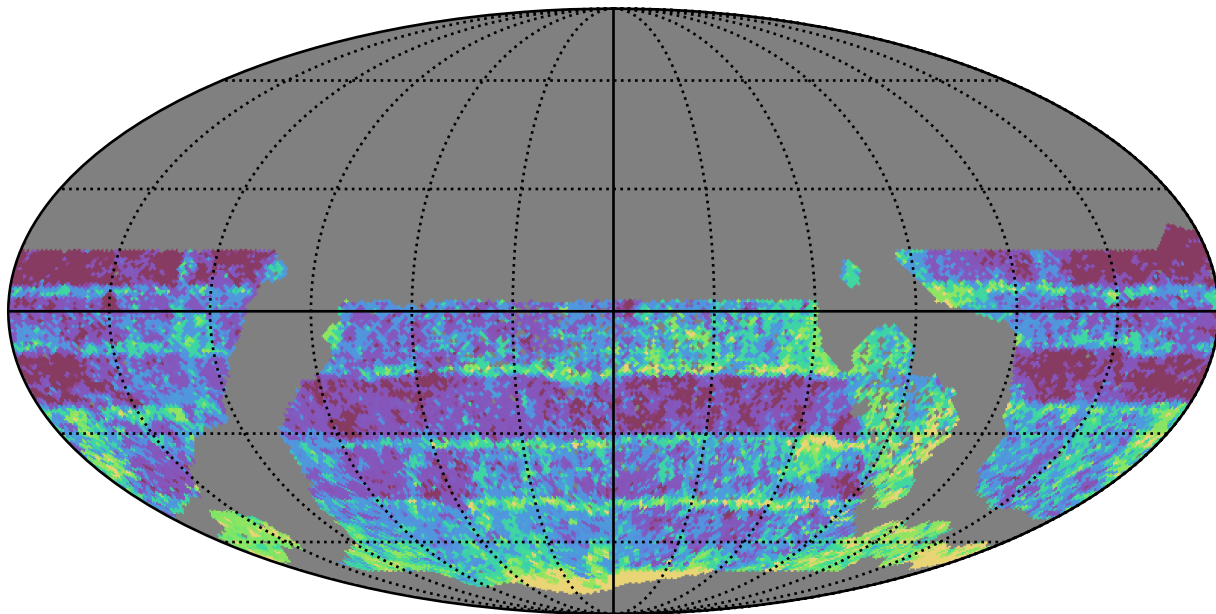
ddf_acor_sf20_lsf30_lsr50_v3.4_10yrs WFD r band: Median Inter-Night Gap
