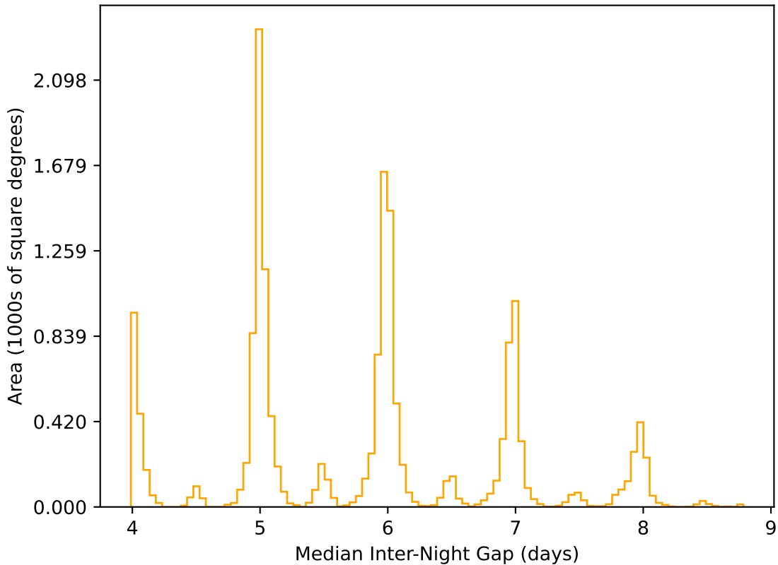
ddf_acor_sf20_lsf30_lsr50_v3.4_10yrs WFD r band: Median Inter-Night Gap
