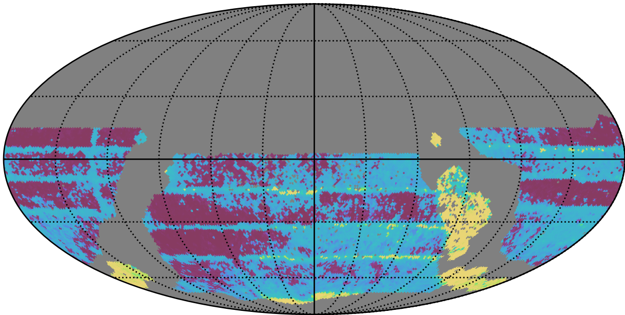
ddf_acor_sf20_lsf30_lsr50_v3.4_10yrs WFD all bands: Median Inter-Night Gap
