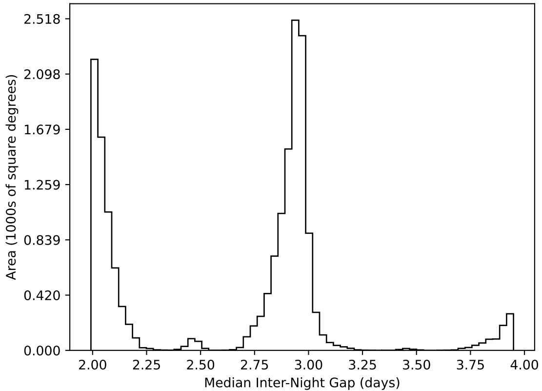
ddf_acor_sf20_lsf30_lsr50_v3.4_10yrs WFD all bands: Median Inter-Night Gap
