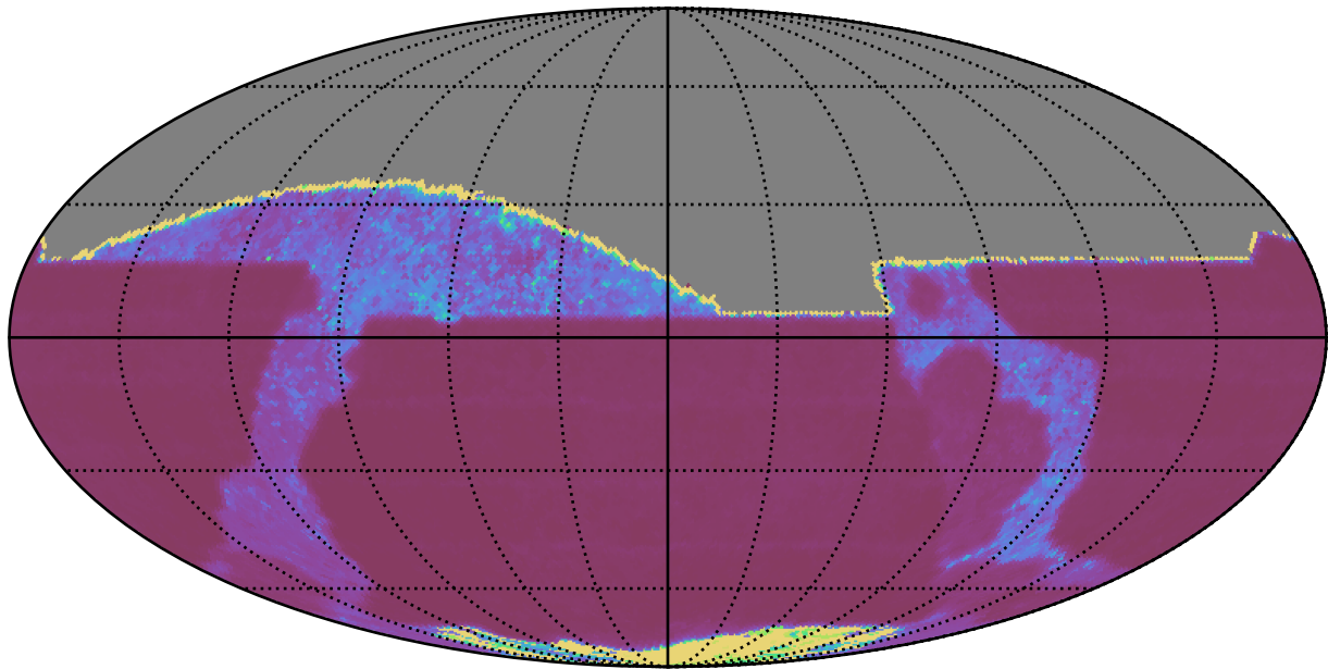
ddf_acor_sf20_lsf30_lsr50_v3.4_10yrs All sky z band: Median Inter-Night Gap
