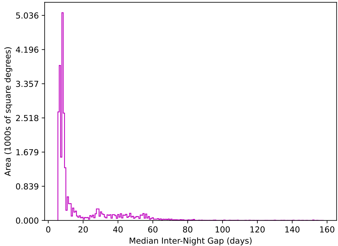
ddf_acor_sf20_lsf30_lsr50_v3.4_10yrs All sky z band: Median Inter-Night Gap
