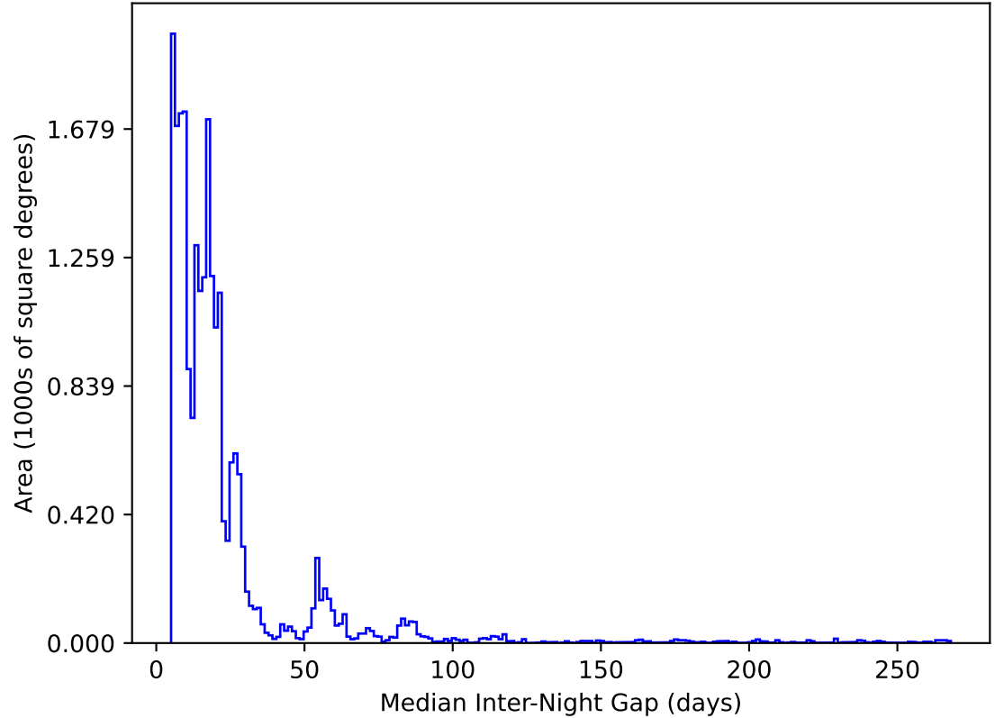
ddf_acor_sf20_lsf30_lsr50_v3.4_10yrs All sky y band: Median Inter-Night Gap
