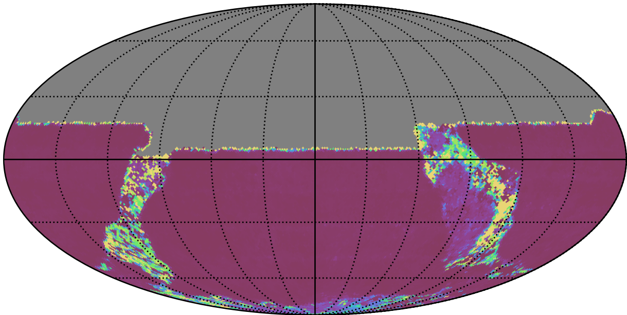
ddf_acor_sf20_lsf30_lsr50_v3.4_10yrs All sky u band: Median Inter-Night Gap
