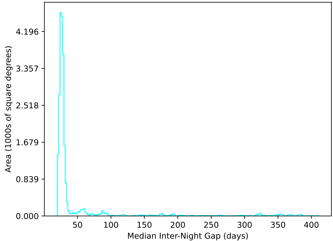
ddf_acor_sf20_lsf30_lsr50_v3.4_10yrs All sky u band: Median Inter-Night Gap
