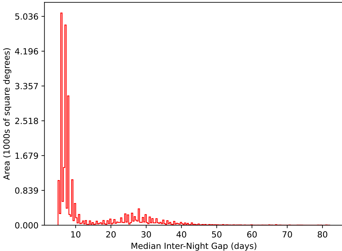
ddf_acor_sf20_lsf30_lsr50_v3.4_10yrs All sky i band: Median Inter-Night Gap
