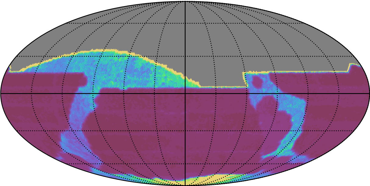
ddf_acor_sf20_lsf30_lsr50_v3.4_10yrs All sky all bands: Median Inter-Night Gap
