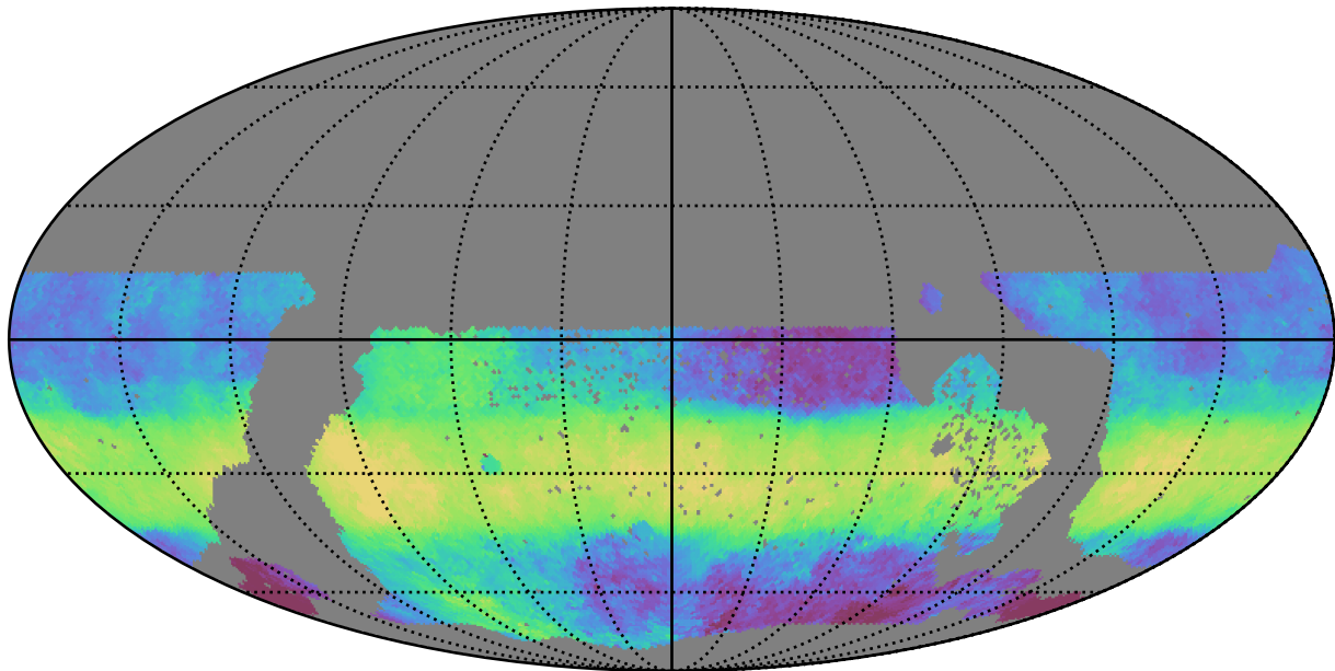
ddf_acor_sf20_lsf30_lsr50_v3.4_10yrs WFD z band: Median HA
