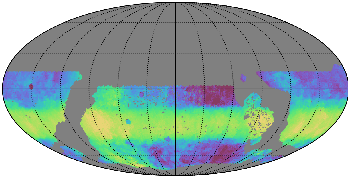
ddf_acor_sf20_lsf30_lsr50_v3.4_10yrs WFD y band: Median HA
