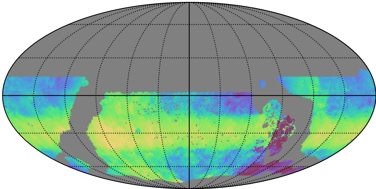
ddf_acor_sf20_lsf30_lsr50_v3.4_10yrs WFD u band: Median HA
