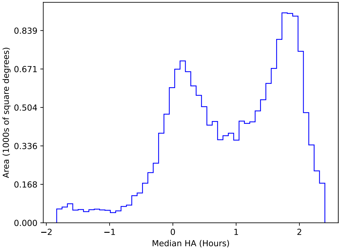
ddf_acor_sf20_lsf30_lsr50_v3.4_10yrs WFD u band: Median HA
