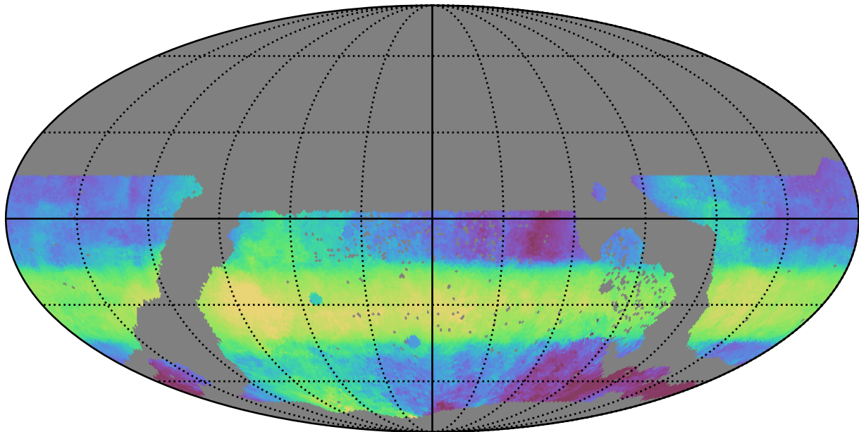
ddf_acor_sf20_lsf30_lsr50_v3.4_10yrs WFD r band: Median HA
