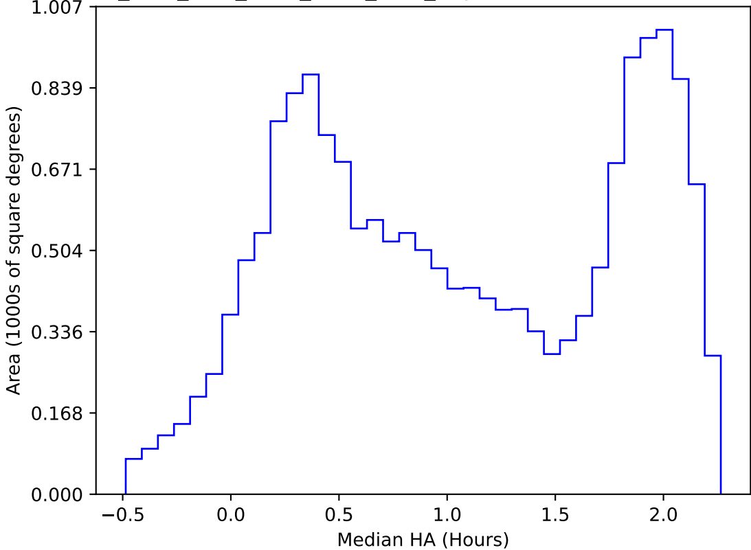
ddf_acor_sf20_lsf30_lsr50_v3.4_10yrs WFD i band: Median HA
