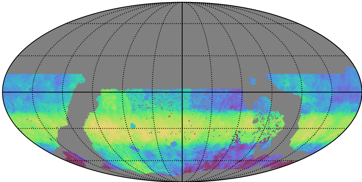
ddf_acor_sf20_lsf30_lsr50_v3.4_10yrs WFD g band: Median HA
