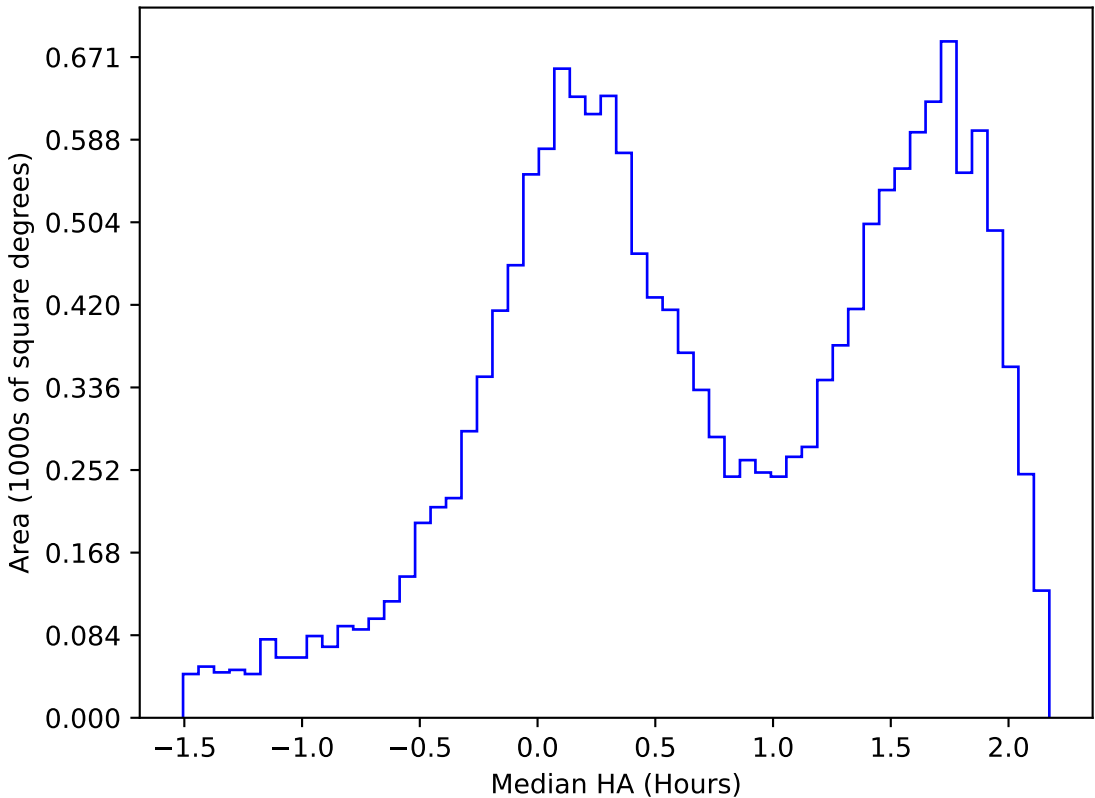
ddf_acor_sf20_lsf30_lsr50_v3.4_10yrs WFD g band: Median HA
