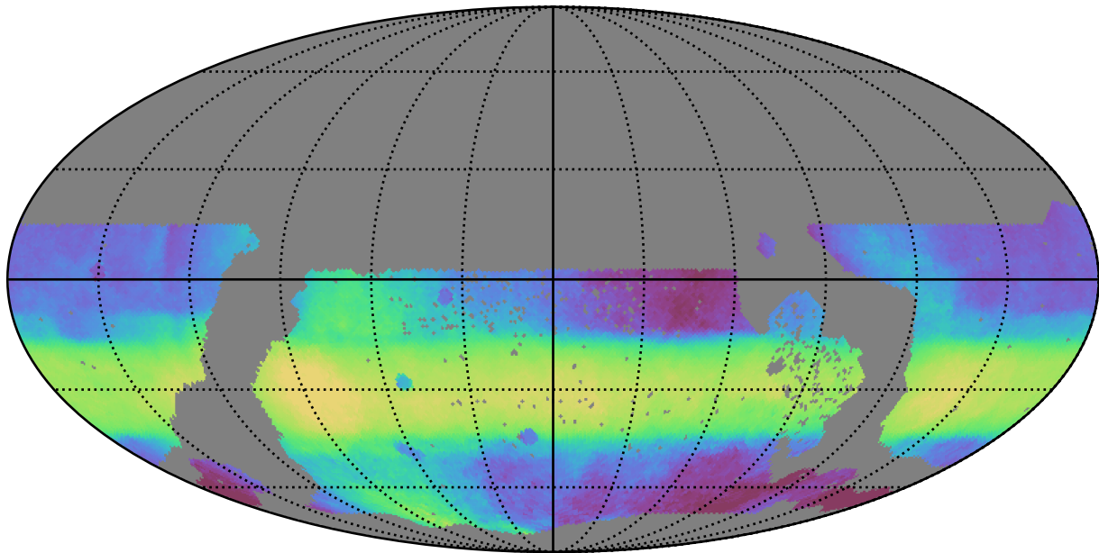
ddf_acor_sf20_lsf30_lsr50_v3.4_10yrs WFD all bands: Median HA
