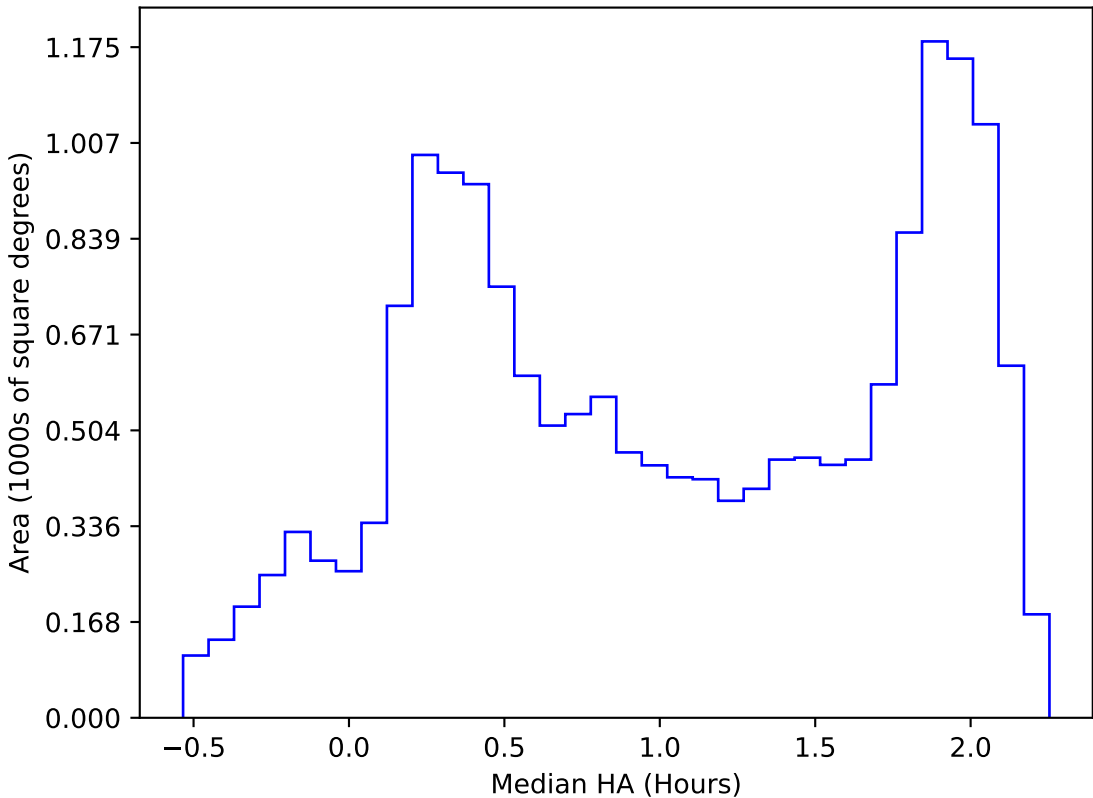
ddf_acor_sf20_lsf30_lsr50_v3.4_10yrs WFD all bands: Median HA
