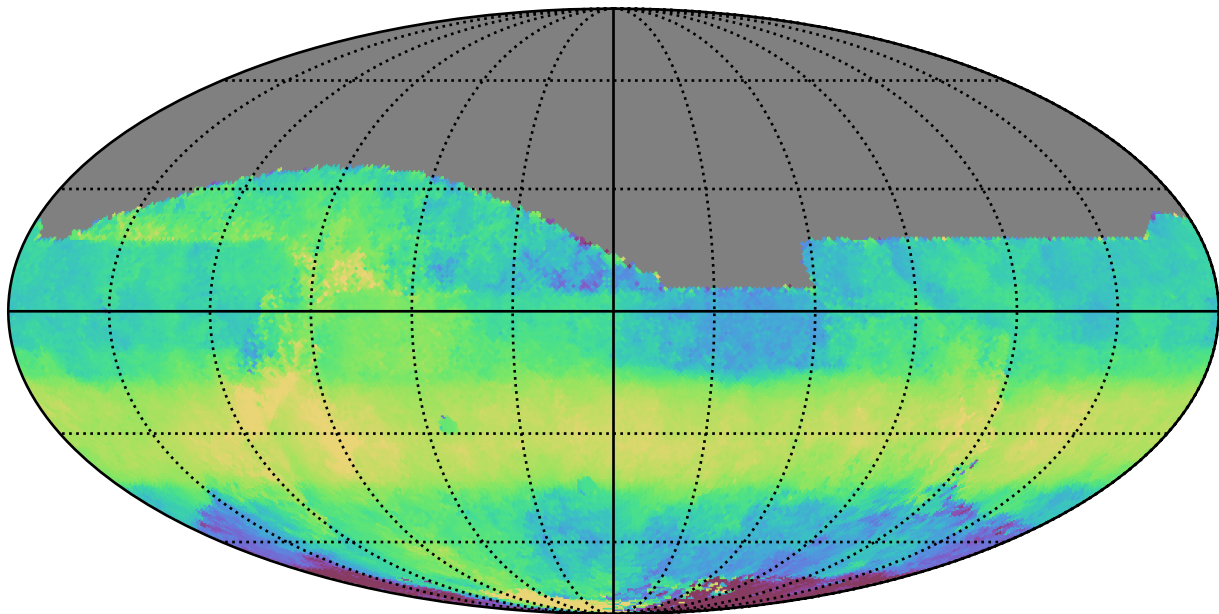
ddf_acor_sf20_lsf30_lsr50_v3.4_10yrs All sky z band: Median HA
