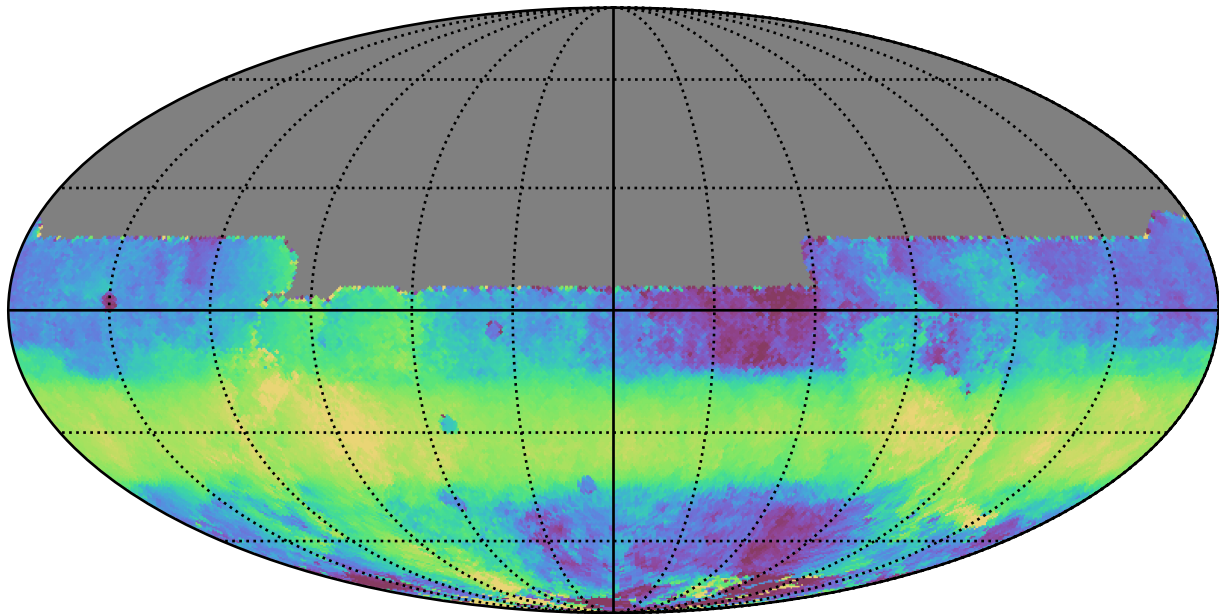
ddf_acor_sf20_lsf30_lsr50_v3.4_10yrs All sky y band: Median HA
