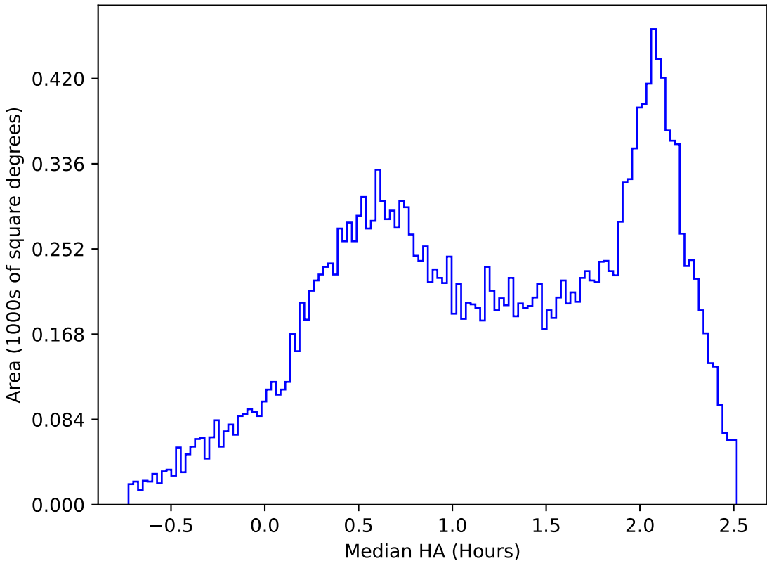
ddf_acor_sf20_ls30_lsr50_v3.4_10yrs All sky y band: Median HA
