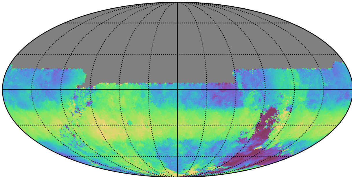
ddf_acor_sf20_lsf30_lsr50_v3.4_10yrs All sky u band: Median HA
