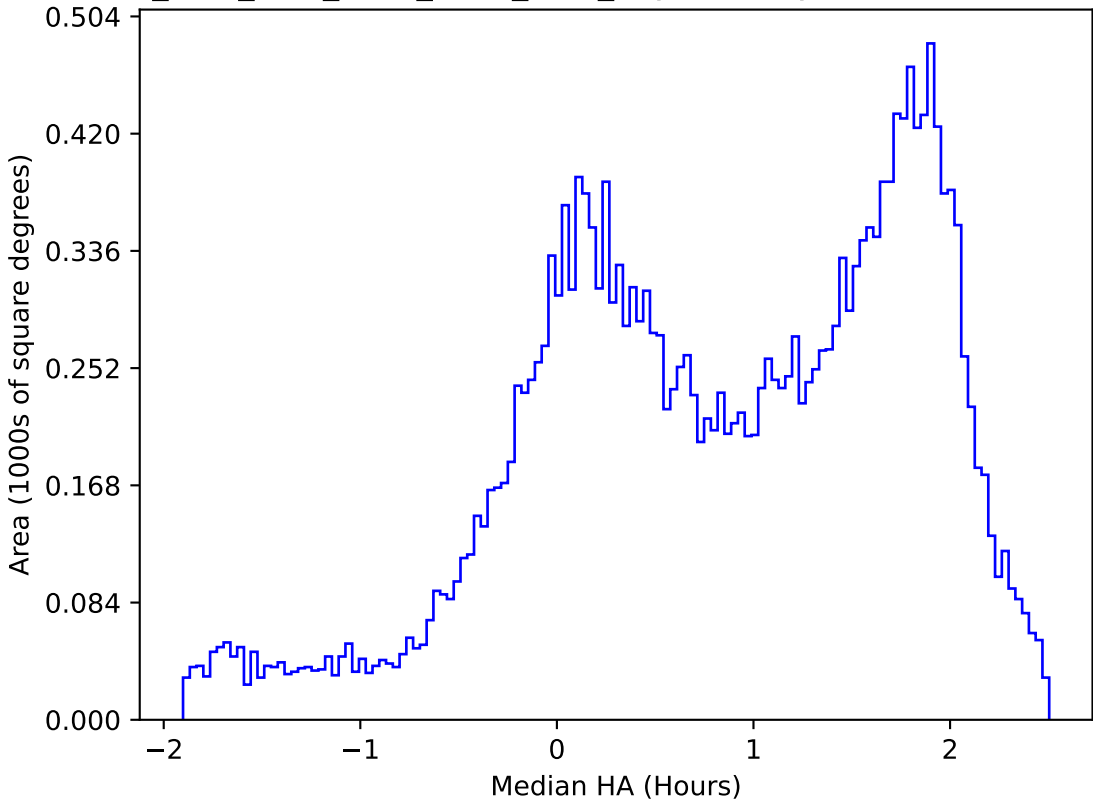
ddf_acor_sf20_ls30_lsr50_v3.4_10yrs All sky u band: Median HA
