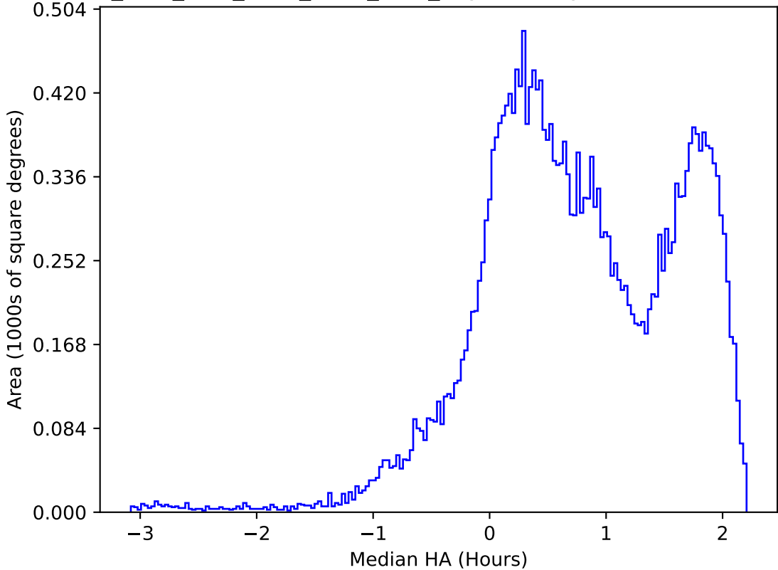
ddf_acor_sf20_lsf30_lsr50_v3.4_10yrs All sky r band: Median HA
