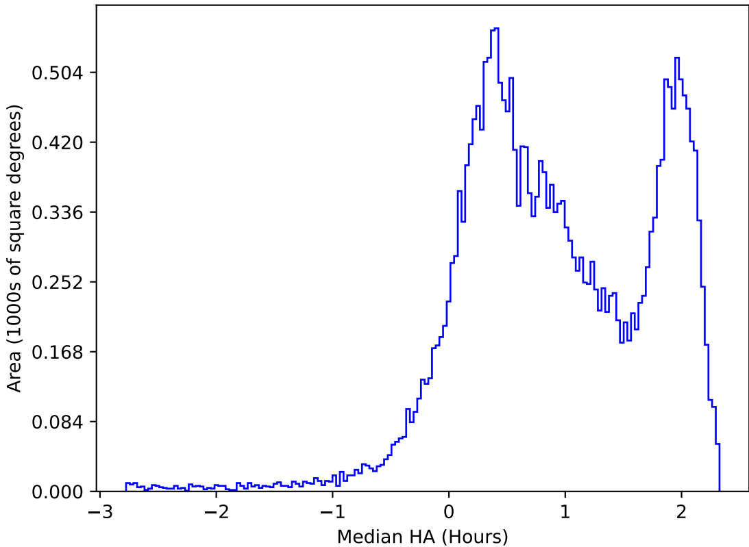
ddf_acor_sf20_lsf30_lsr50_v3.4_10yrs All sky i band: Median HA
