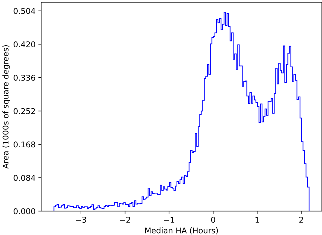
ddf_acor_sf20_ls30_lsr50_v3.4_10yrs All sky g band: Median HA
