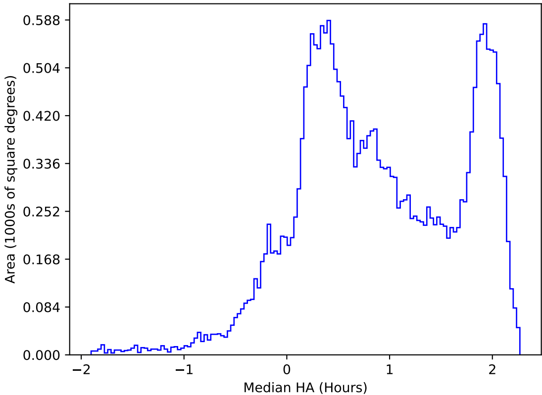
ddf_acor_sf20_lsf30_lsr50_v3.4_10yrs All sky all bands: Median HA
