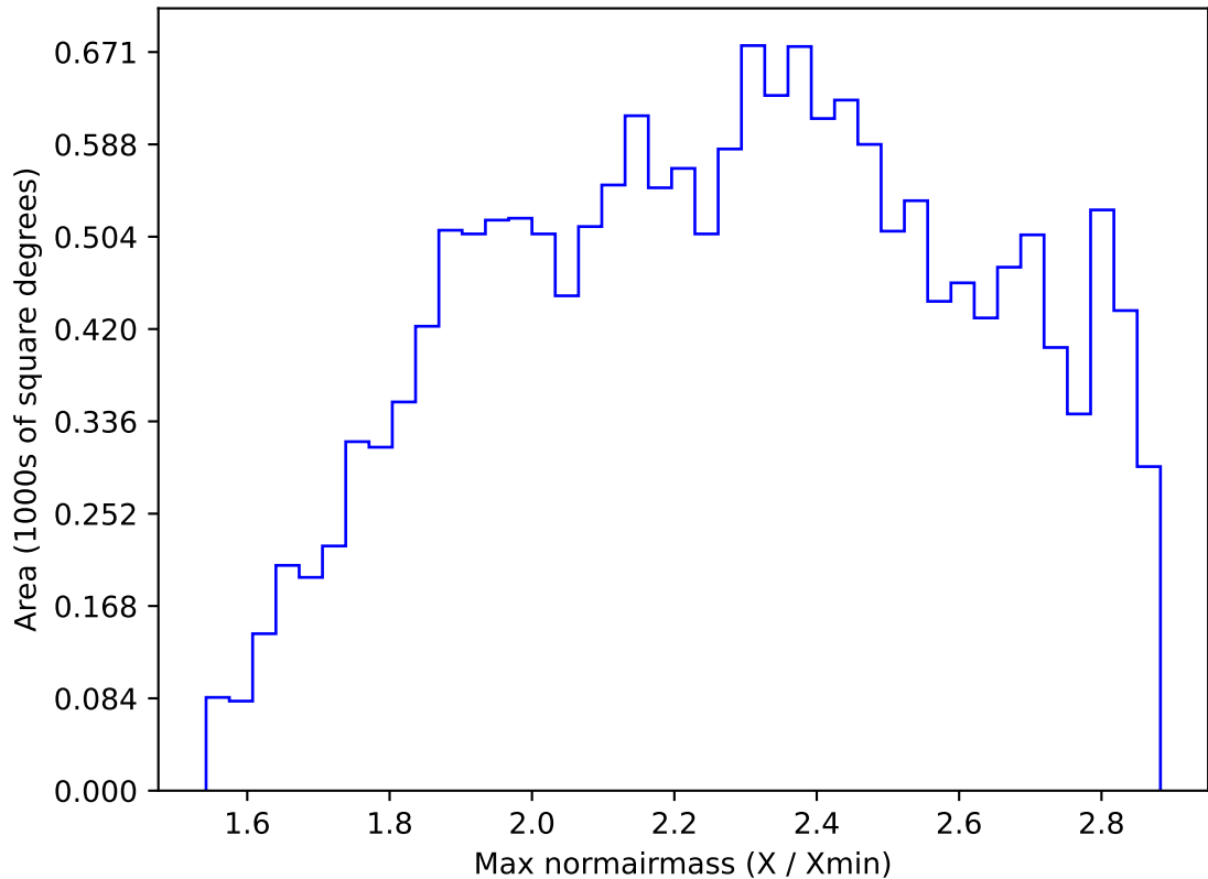
ddf_acor_sf20_lsf30_lsr50_v3.4_10yrs WFD i band: Max normairmass
