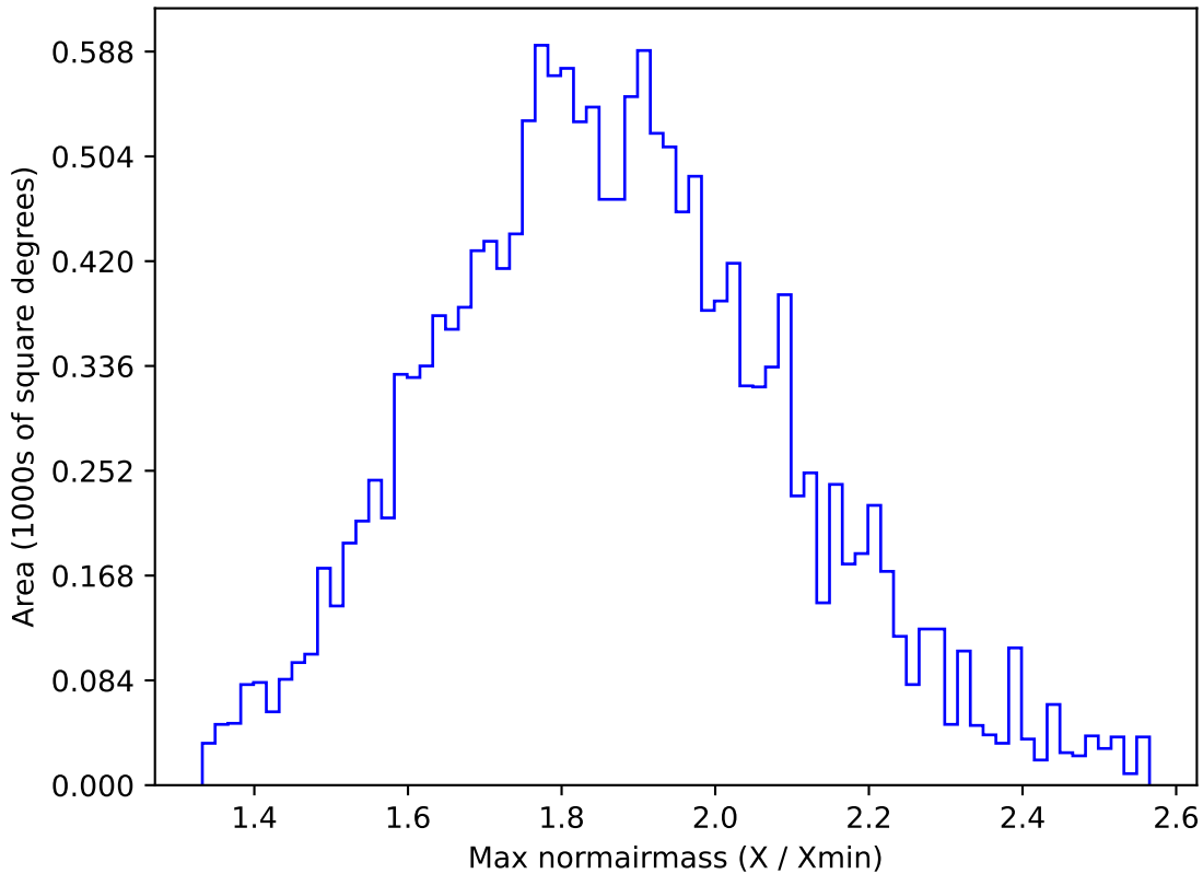
ddf_acor_sf20_lsf30_lsr50_v3.4_10yrs WFD g band: Max normairmass
