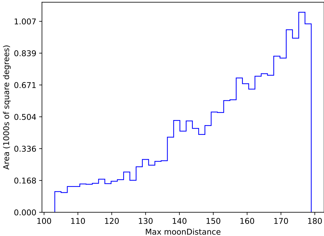
ddf_acor_sf20_lsf30_lsr50_v3.4_10yrs WFD z band: Max moonDistance
