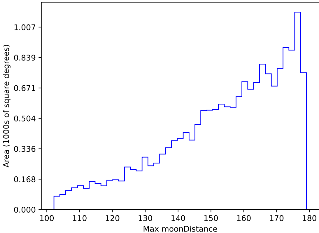
ddf_acor_sf20_lsf30_lsr50_v3.4_10yrs WFD u band: Max moonDistance
