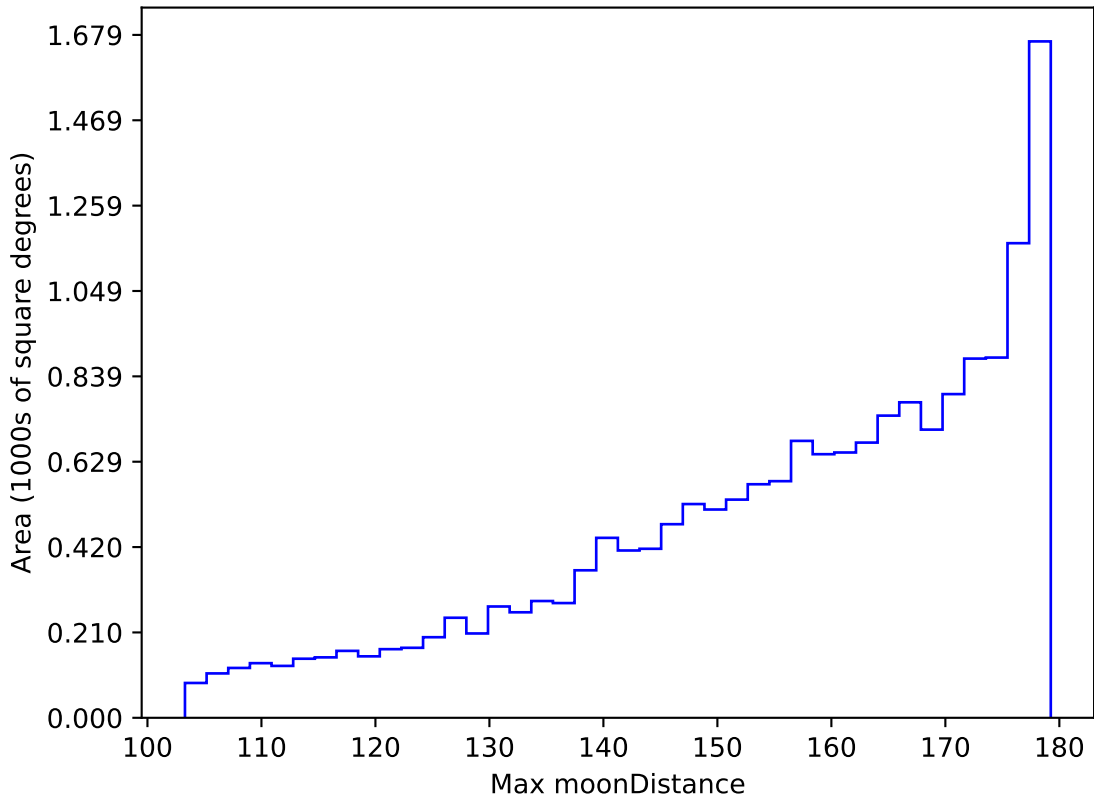
ddf_acor_sf20_lsf30_lsr50_v3.4_10yrs WFD r band: Max moonDistance
