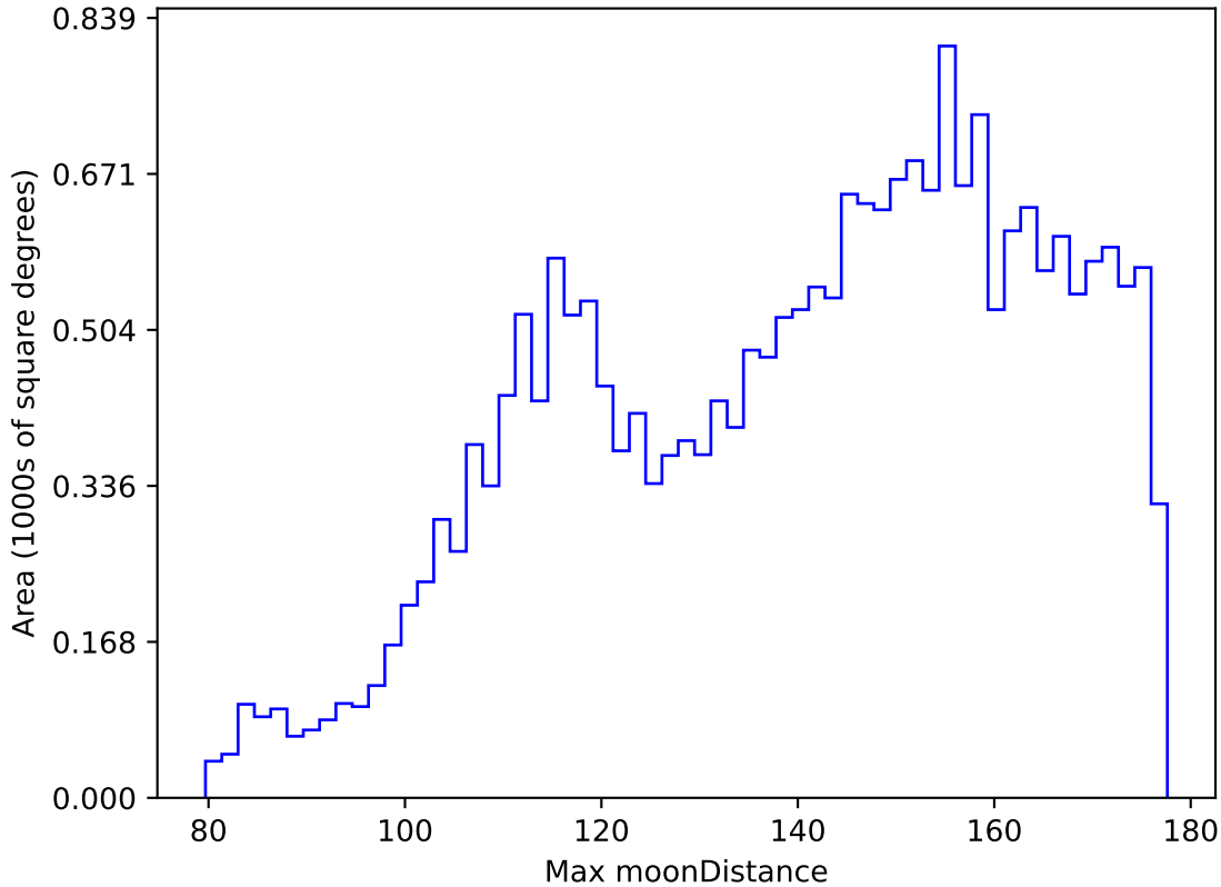
ddf_acor_sf20_lsf30_lsr50_v3.4_10yrs All sky y band: Max moonDistance
