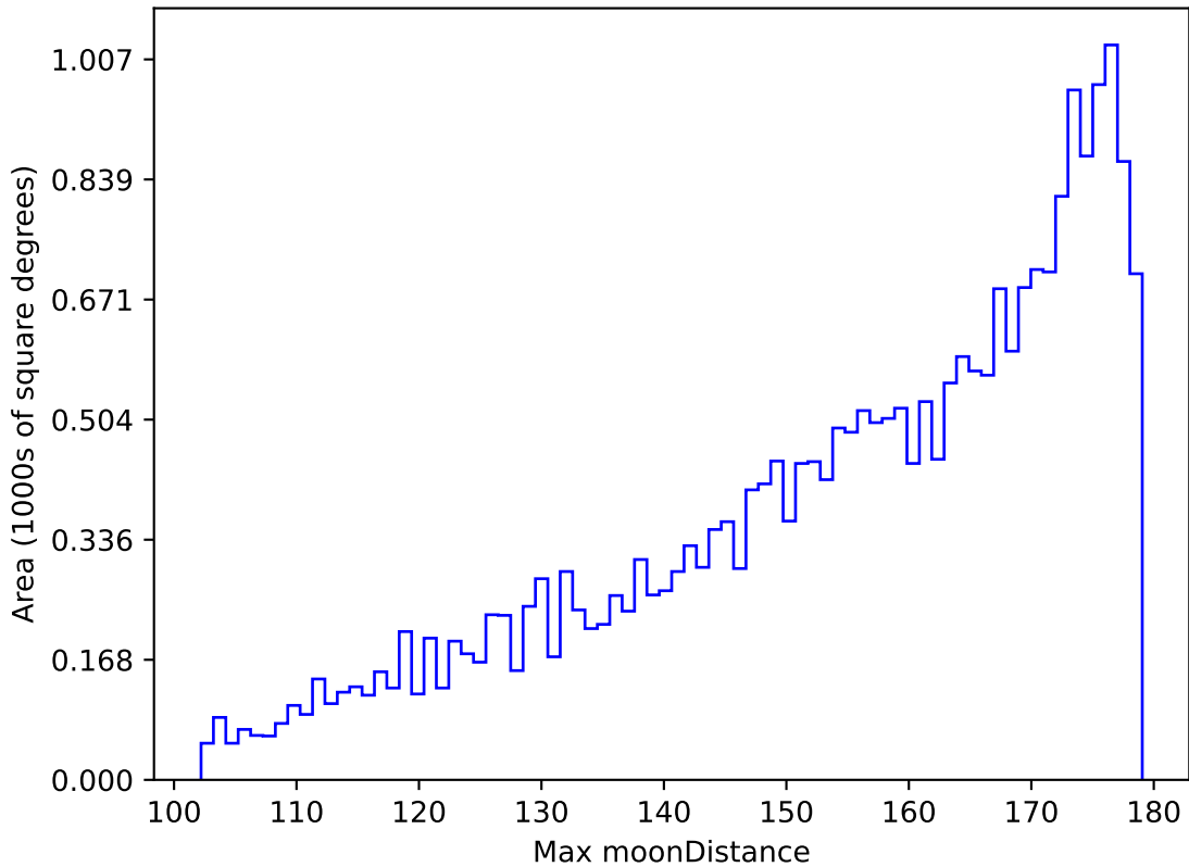
ddf_acor_sf20_lsf30_lsr50_v3.4_10yrs All sky g band: Max moonDistance
