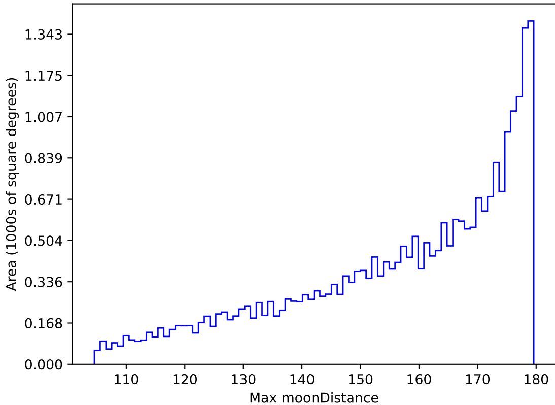
ddf_acor_sf20_lsf30_lsr50_v3.4_10yrs All sky all bands: Max moonDistance
