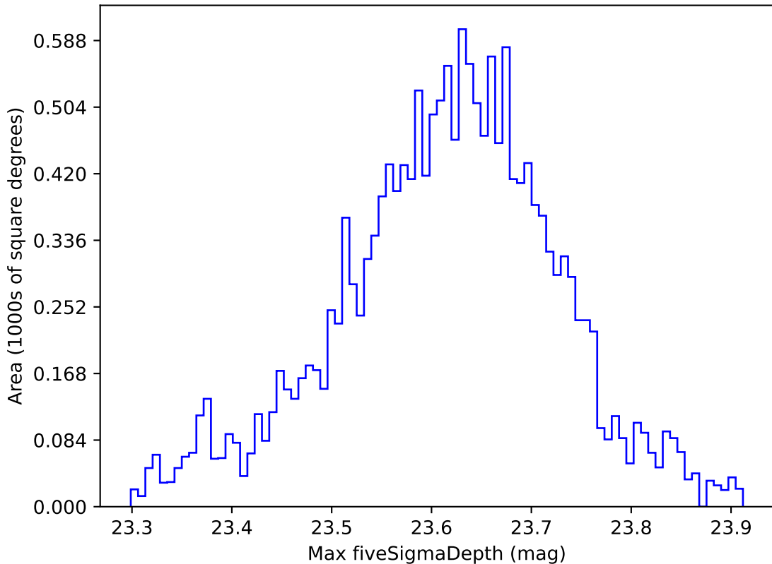
ddf_acor_sf20_lsf30_lsr50_v3.4_10yrs WFD z band: Max fiveSigmaDepth
