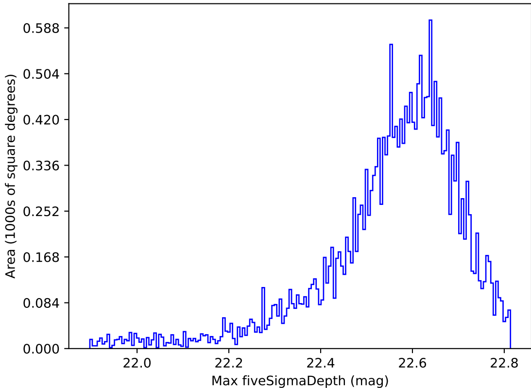
ddf_acor_sf20_lsf30_lsr50_v3.4_10yrs All sky y band: Max fiveSigmaDepth
